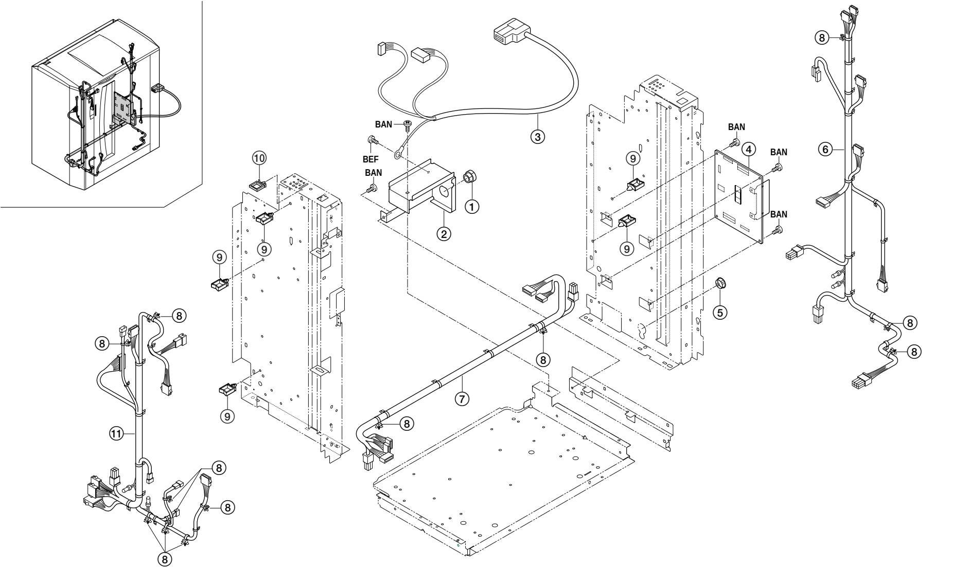
FIG. 4 ELECTRICAL COMPONENTS
