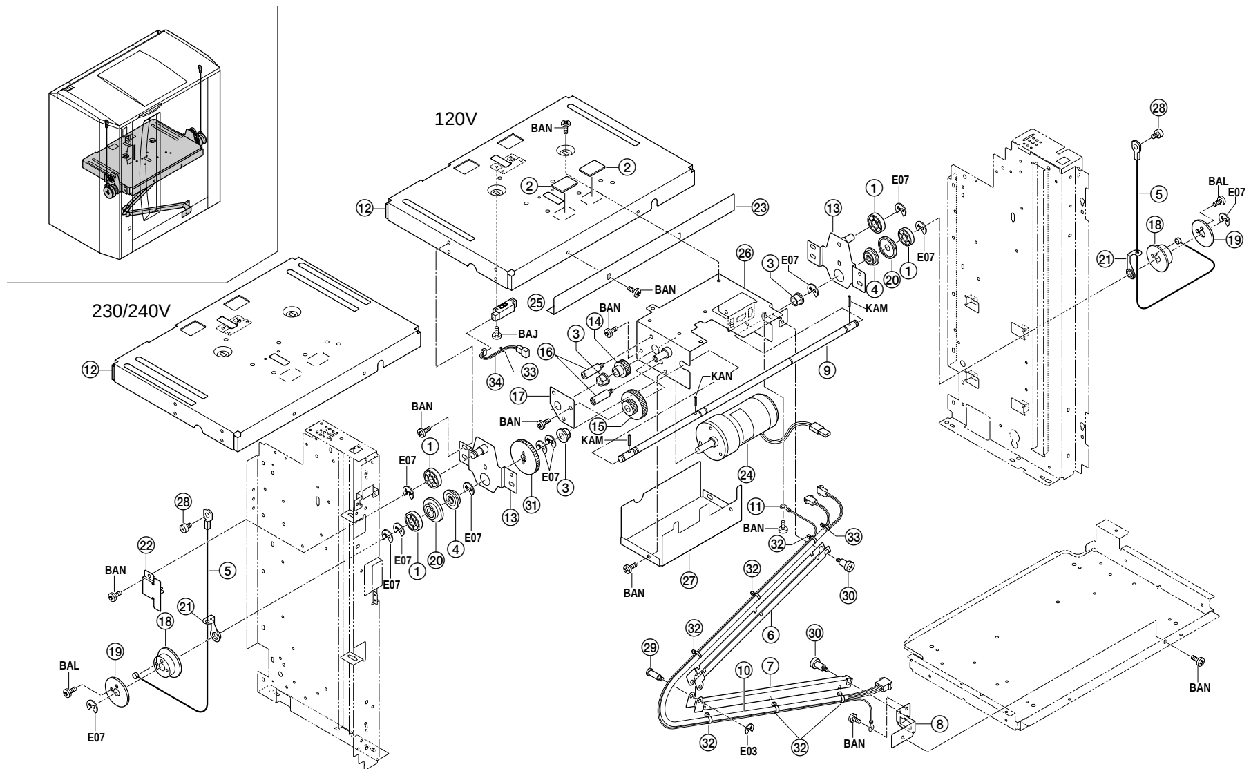
FIG. 2 LIFT PLATE SECTION
