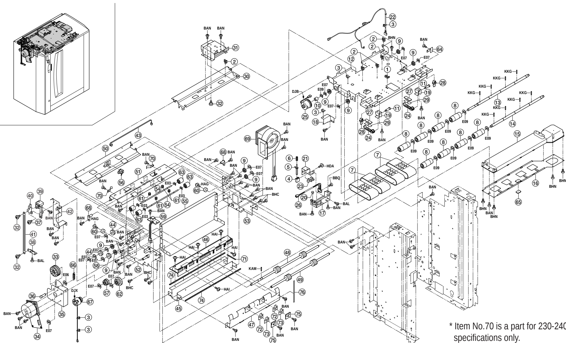
FIG. 3 PAPER FEED-IN SECTION
